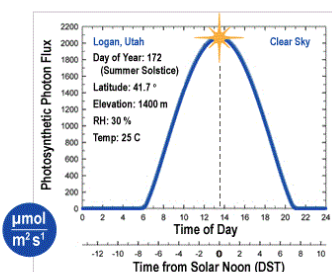
MODEL FOR QUANTUM SENSOR PHOTOSYNTHETIC PHOTON FLUX
